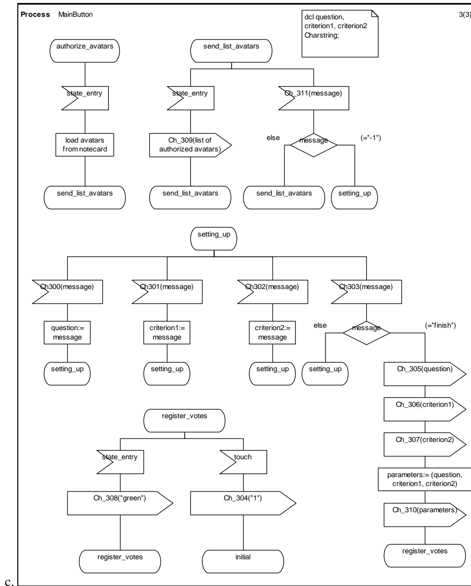
Figure 10.3. SDL model of the script controlling the MainButton of the VotingFloor .
